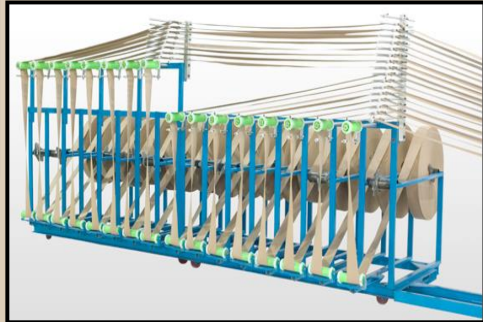
32 Layer (16 + 16) Reel Stands and Cascade Glue Tanks
